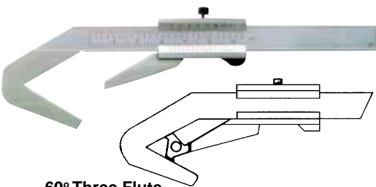
60° Three Flute
